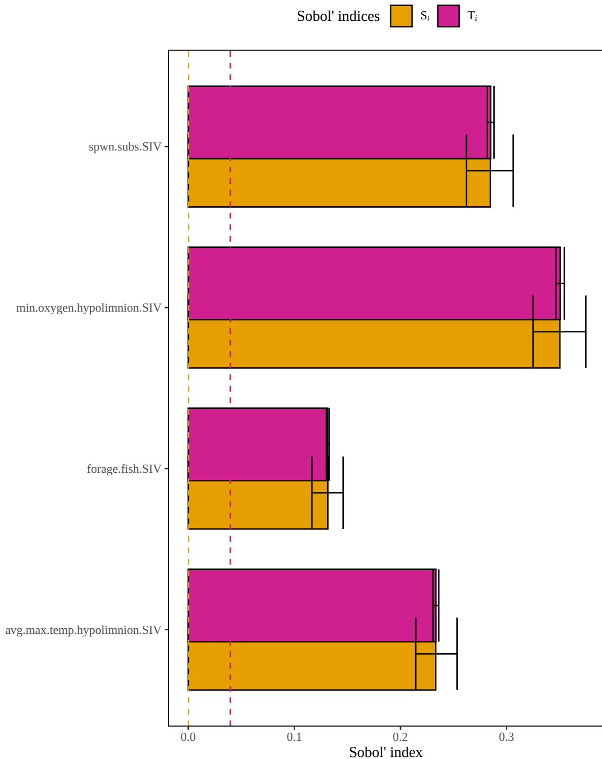
Figure 4. Results of a sensitivity analysis for the laketroutReproducingLakes model based on an arithmetic mean structure. Dashed lines represent baseline numerical approximation error for S_i and T_i ( i.e. , dummy variables).
